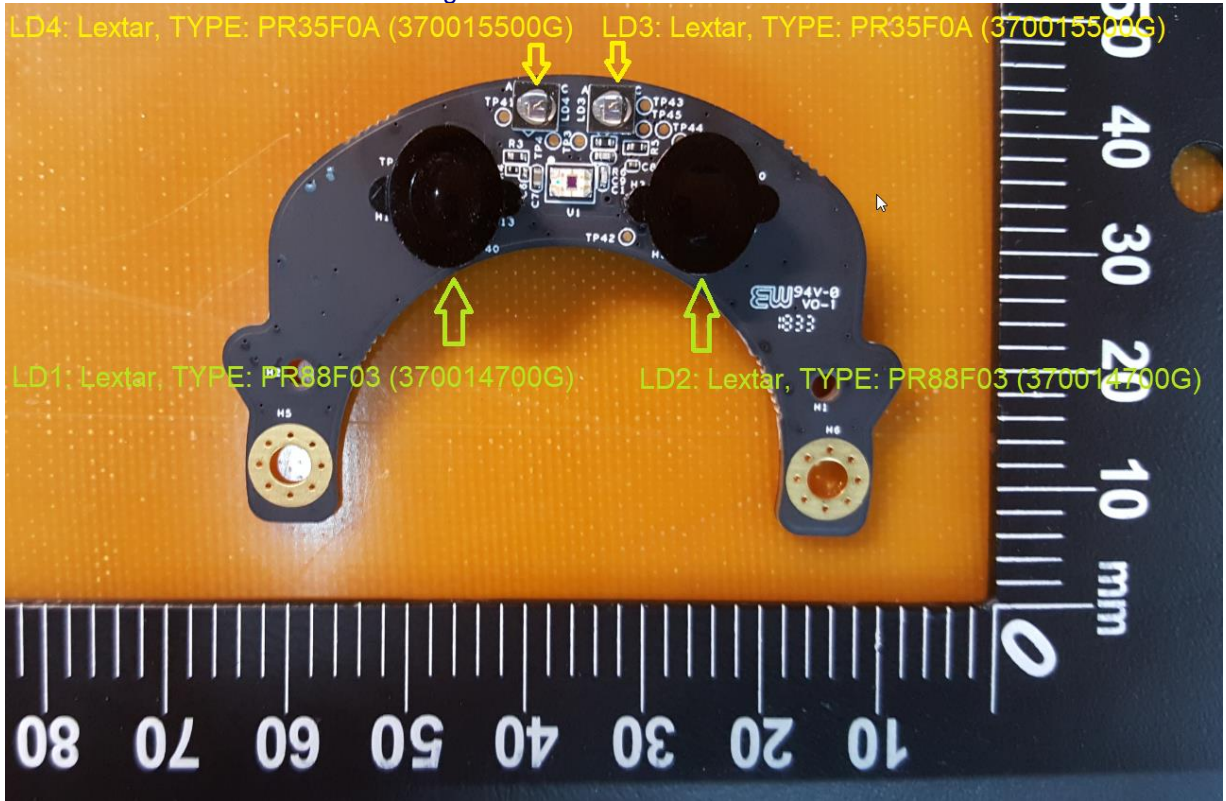
Fig.10: Remote LED board view-2
