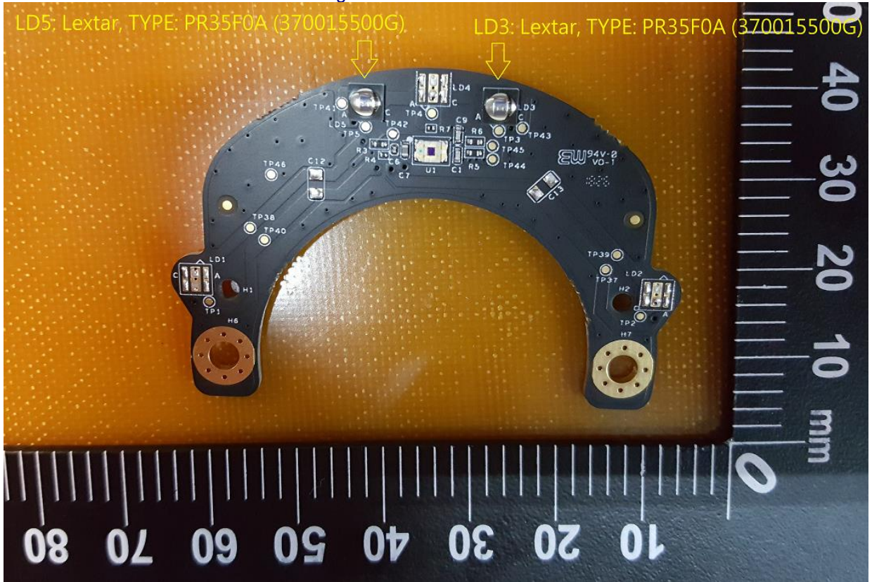
Fig.4: Fix LED board view-2
