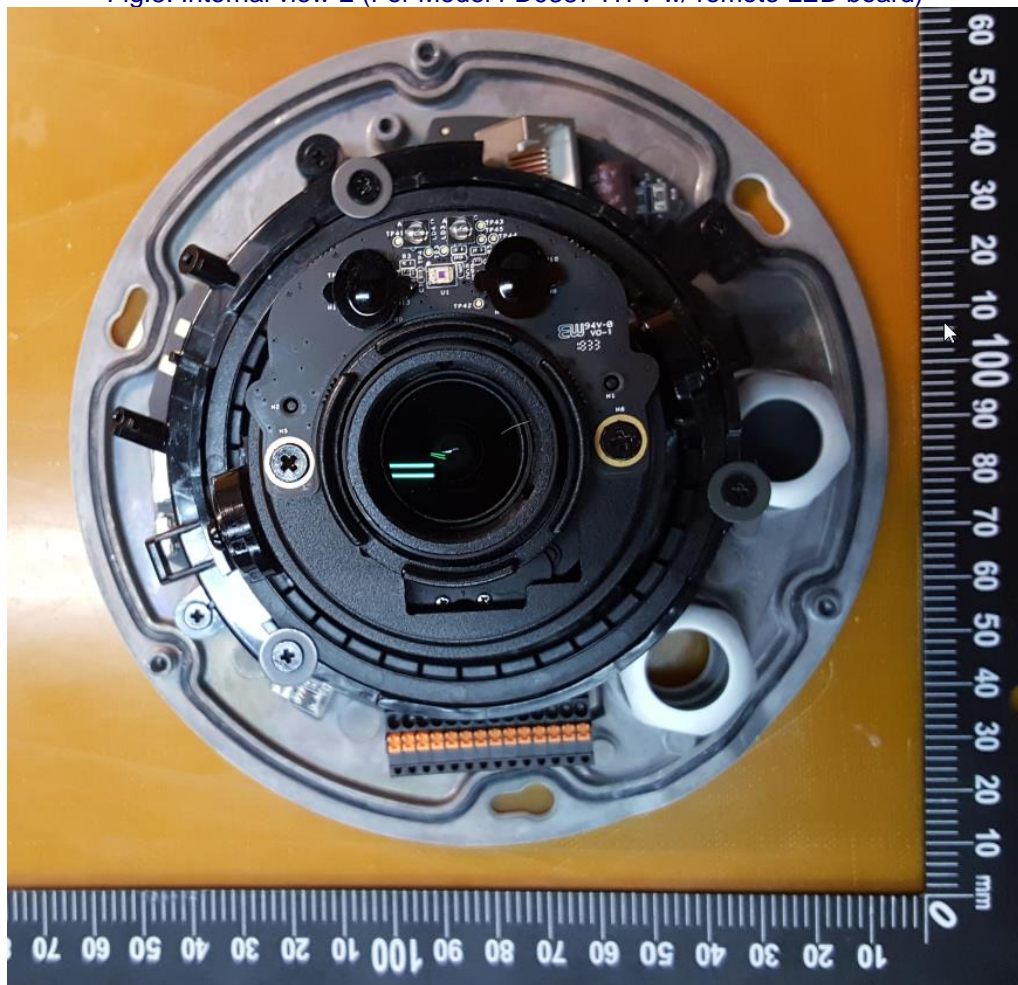
Fig.8: Internal view-2 (For Model FD9387-HTV w/ remote LED board)
