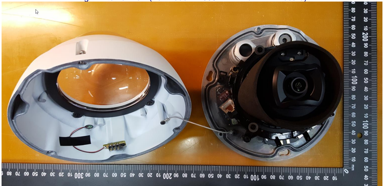
Fig.2: Internal view (For Model FD9387-EHV w/ fix LED board)
