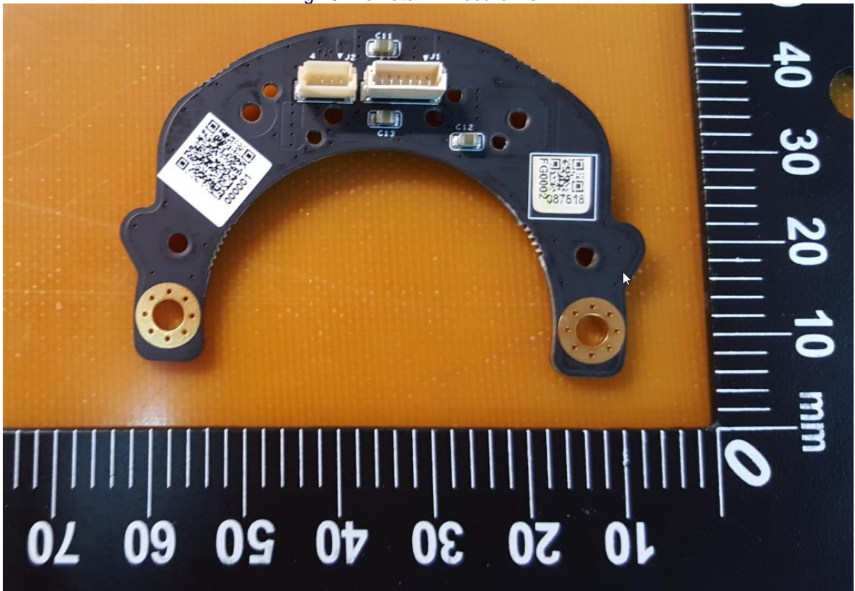
Fig.10: Remote LED board view-2
