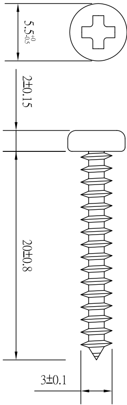
M3 x 20 Hardware Installation
