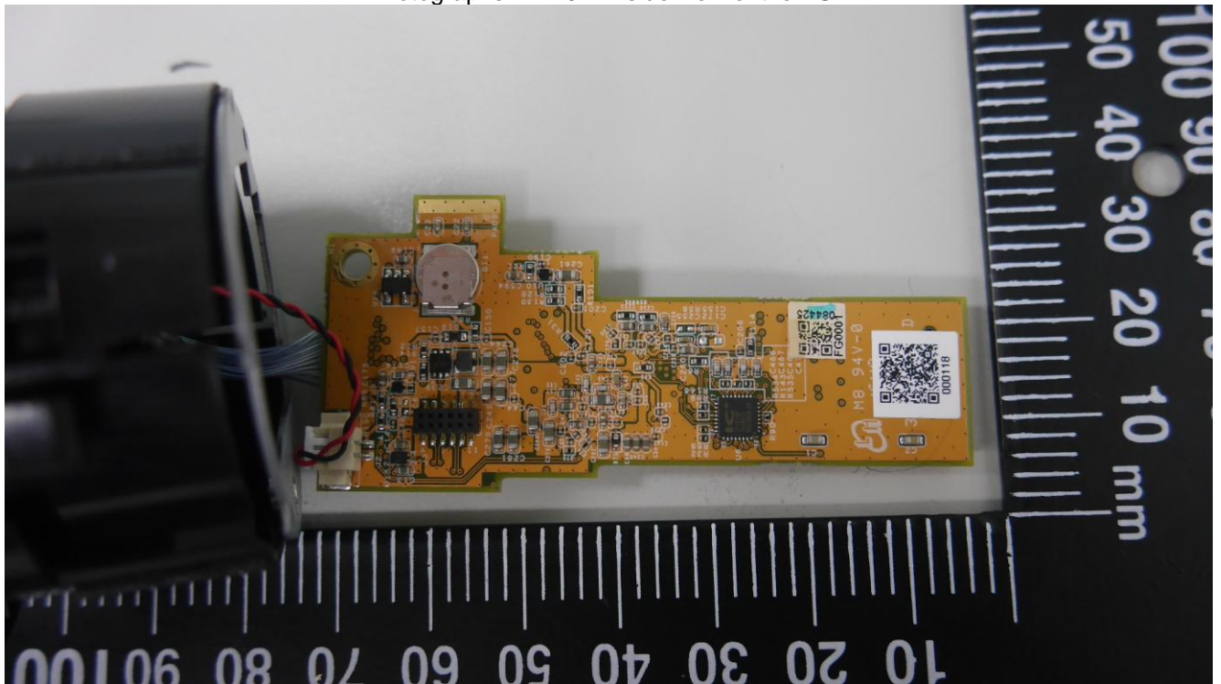
Photographs ID 1-07: Inside view of the EUT
