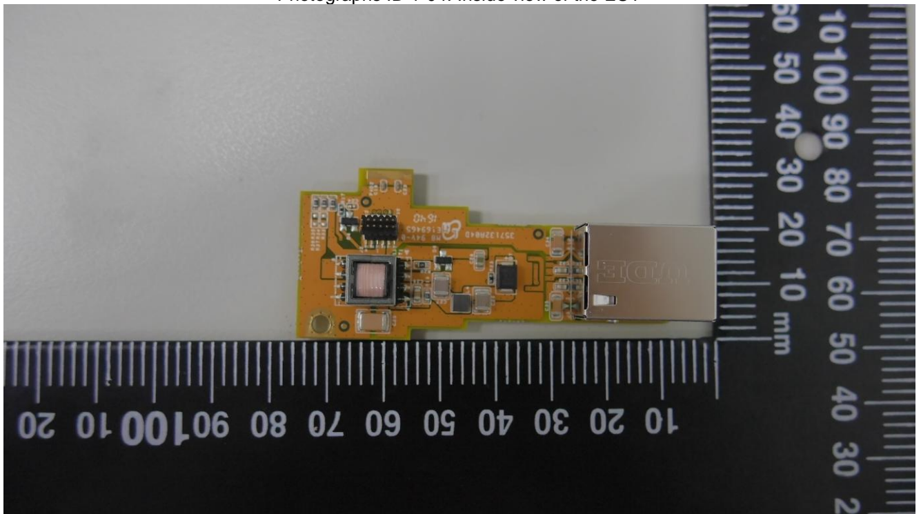
Photographs ID 1-04: Inside view of the EUT
