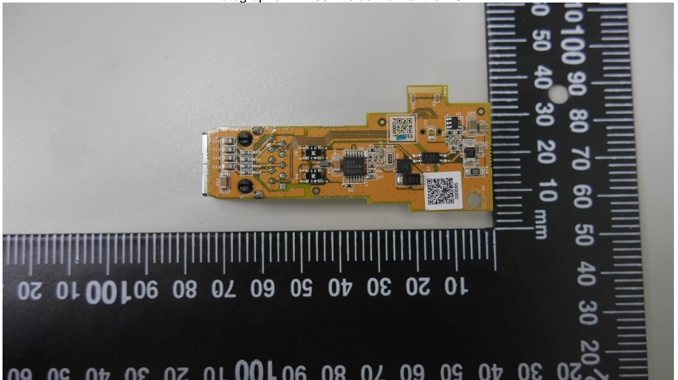
Photographs ID 1-06: Inside view of the EUT
