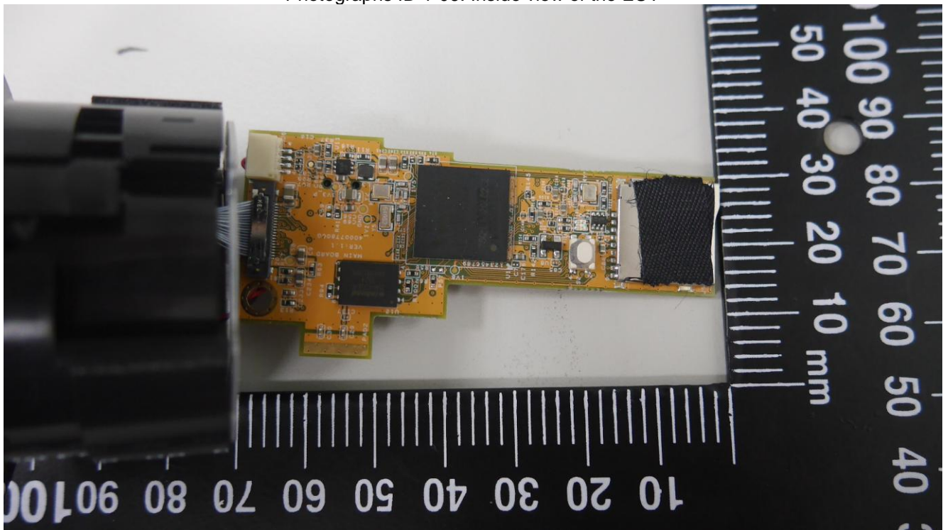
Photographs ID 1-06: Inside view of the EUT
