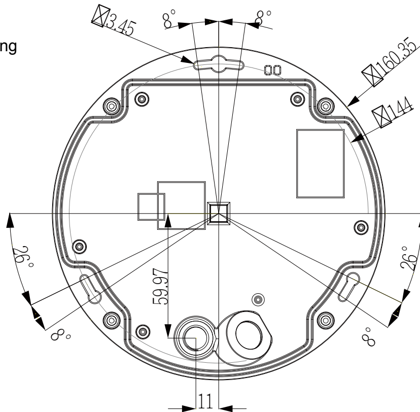
Camera Mounting Plate Mounting Positions
