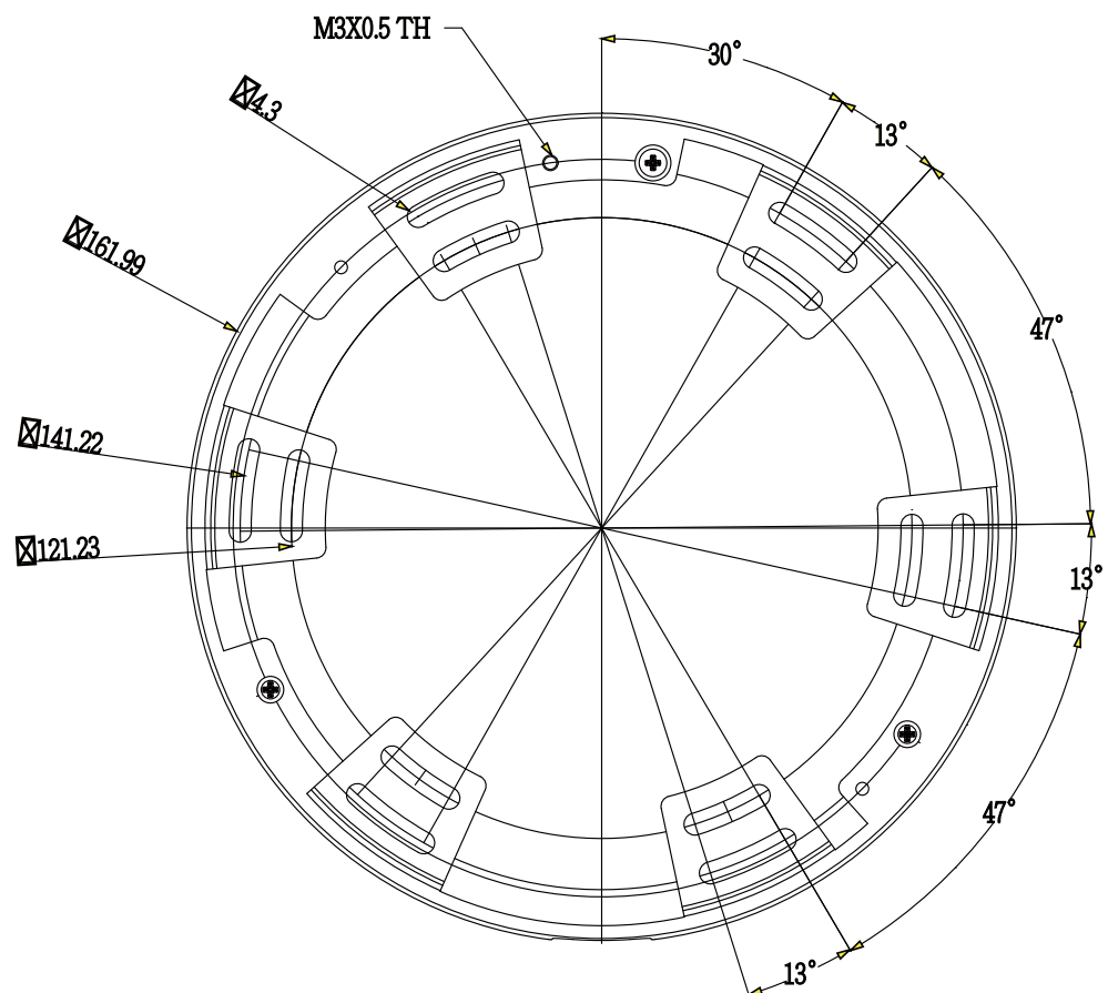
Camera Mounting Plate Mounting Positions
